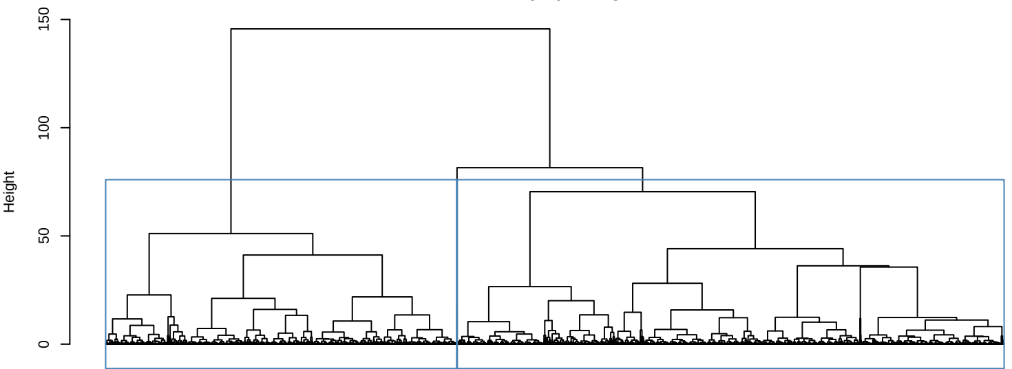
Ward (D2) linkage
