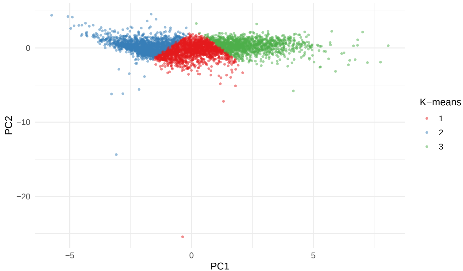
K-means clusters (k = 3) in PC1–PC2
