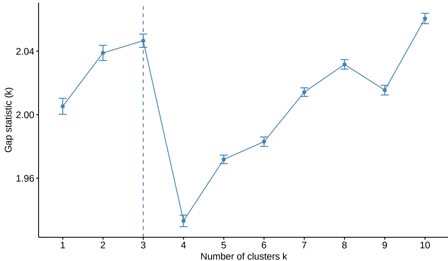
Gap statistic — Tibshirani 2001 SEmax rule
