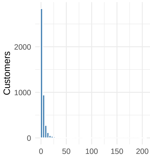
Frequency
