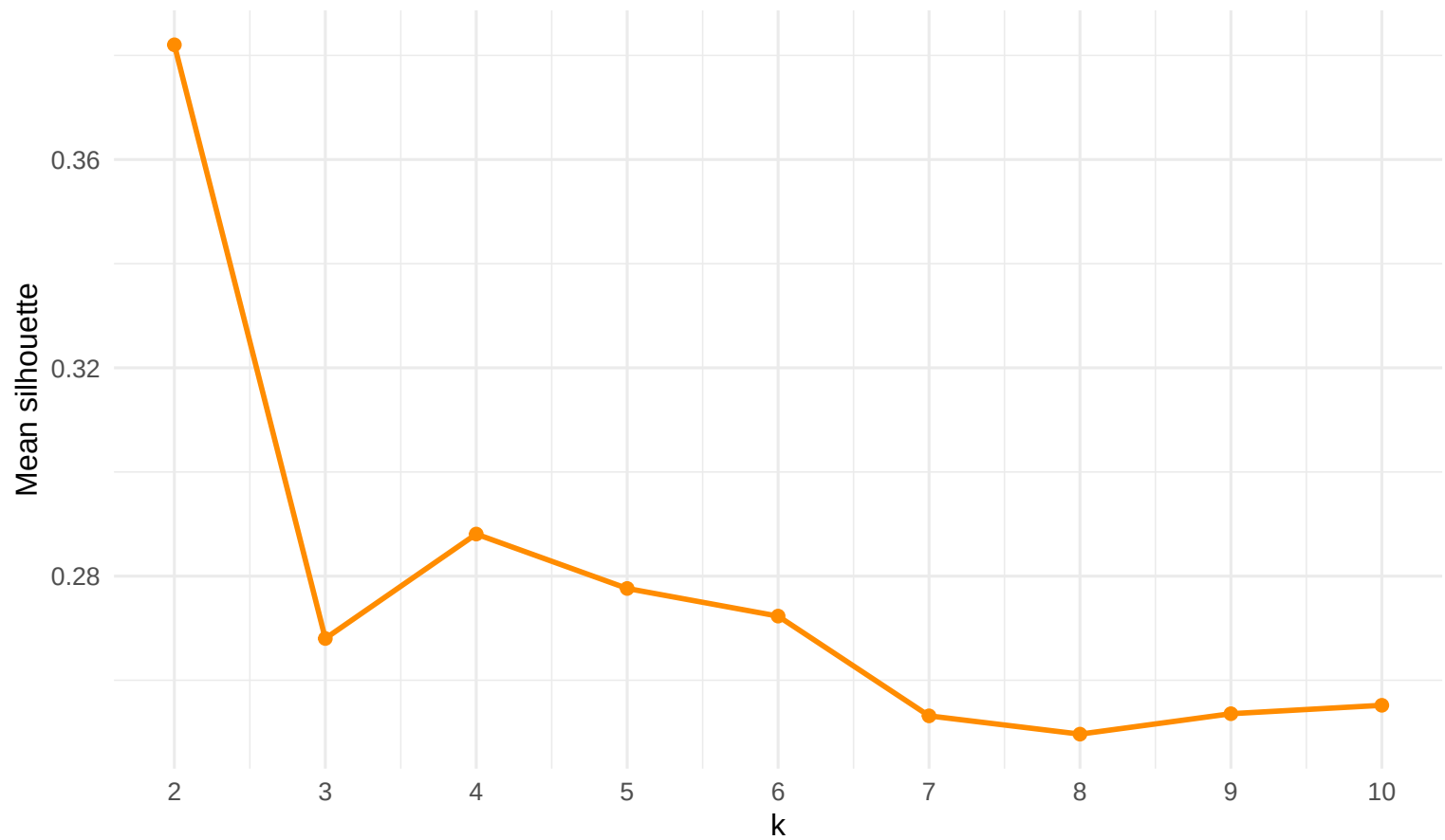
K-means: average silhouette vs k
