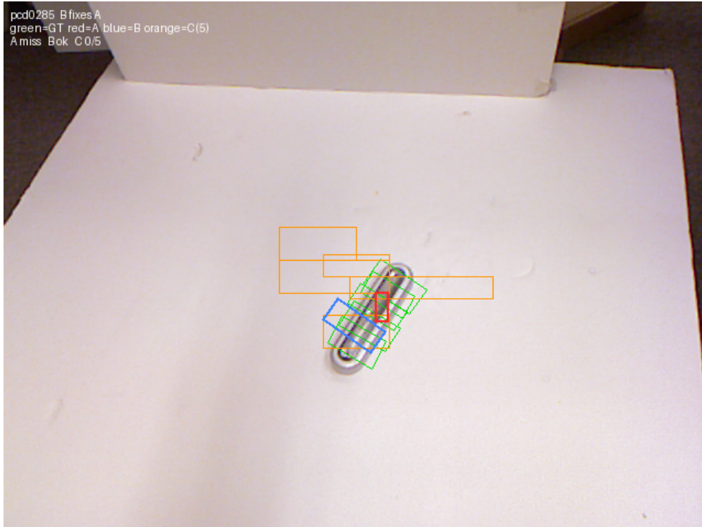
Fig. 5. All three systems on one image. Labeled ground-truth grasps are green, System A red, System B blue, and System C's five repeats orange.
