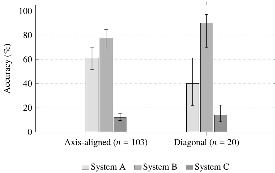
Fig. 4. Accuracy by orientation stratum with 95% Wilson intervals. Axis-aligned, 103 images: System A 61.2 [51.5, 70.0], System B 77.7 [68.7, 84.6], System C 12.0 [9.5, 15.1]. Diagonal, 20 images: System A 40.0 [21.9, 61.3], System B 90.0 [69.9, 97.2], System C 14.0 [8.5, 22.1]. These are image-level rather than object-clustered, so they are the narrower reading. The three systems move in three directions, but the diagonal intervals are already wide enough that only System A's drop, which was predicted from its representation beforehand, should carry weight.
