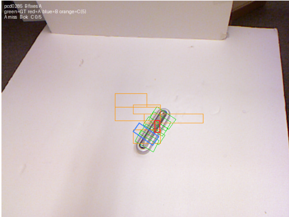
Fig. 4. All three systems on one image. Labeled ground-truth grasps are green, System A red, System B blue, and System C's five repeats orange.
