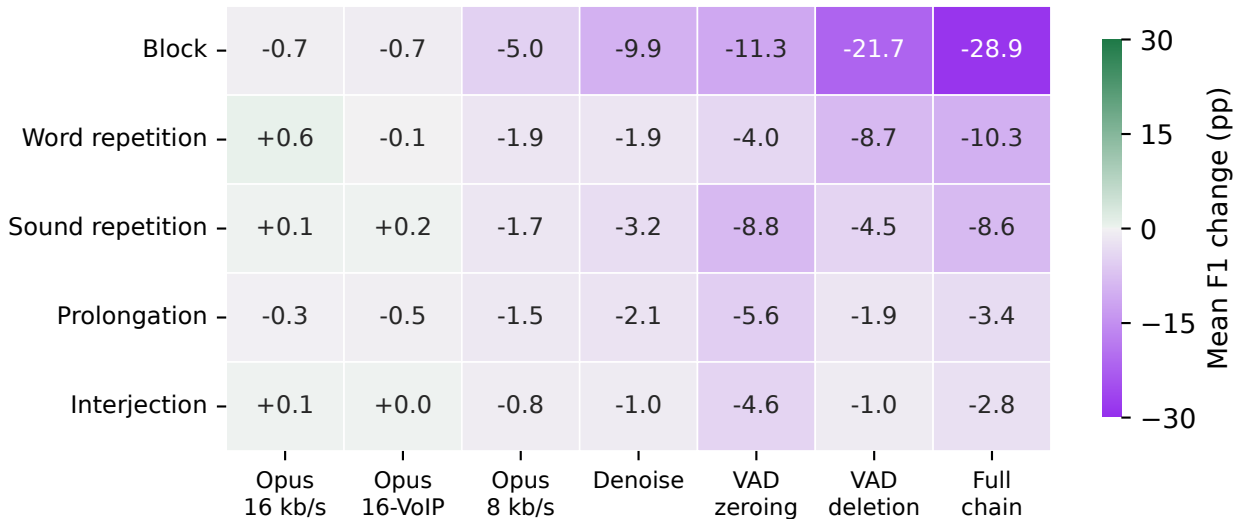
Mean F1 change versus clean (percentage points): positive = improvement
