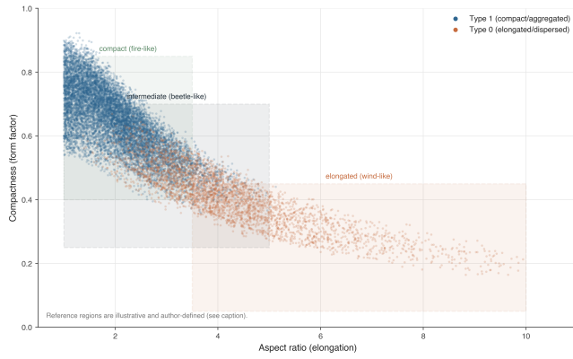
Figure 9: Shape-space scatter (compactness vs. aspect ratio) per endpoint, with illustrative , author-defined shape regions overlaid. The separation is partly circular because aspect ratio defines the gradient and compactness is coupled to it; the regions are not published per-agent envelopes.
