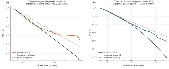
Figure 8: Complementary cumulative distribution functions (CCDF) of cluster size ( n ) per endpoint. Both are better described by a lognormal than a power law; Type1 has the heavier upper tail, consistent with its larger mean cluster area.
