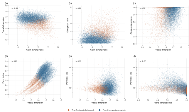
Figure 4: Pairwise scatter plots of selected spatial metrics, coloured by morphological type.
