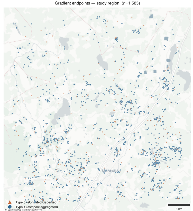
Figure 7: Spatial distribution of the two gradient endpoints within a southern display window (one tile, 10.9% of clusters, shown for legibility). Blue circles: Type 1 (compact/aggregated); brown triangles: Type 0 (elongated/dispersed). Inset: all 14,582 clusters sampled across Finland for geographic context.
