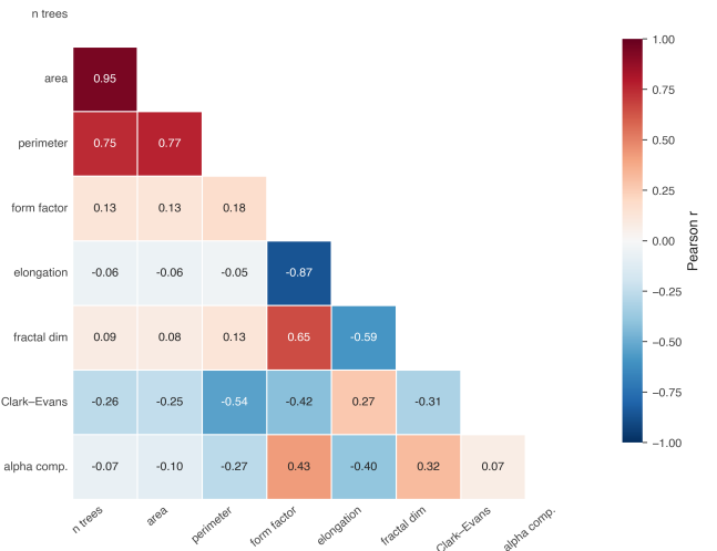
Figure 3: Correlation matrix for cluster-level spatial metrics.
