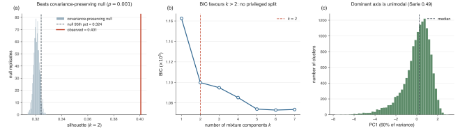
Figure 6: Significance and discreteness of the k = 2 partition. (a) The observed silhouette (red line, 0.401) exceeds a 999-replicate covariance-preserving null (single multivariate Gaussian matched to the feature covariance; mean 0.321, 95th pct 0.324), p = 0.001 —a far stricter test than column-shuffling. (b) Gaussian-mixture BIC decreases monotonically past k = 2 , so no two-component model is privileged. (c) The first principal component (60% of variance) is unimodal (Sarle coefficient 0.486). Together: real structure, but a continuous gradient rather than two discrete classes.
