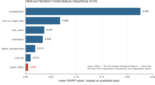
Figure 13: Mean |\text{SHAP}| feature importance for the held-out Random Forest (E10). Compactness dominates; reach.200m (the only shape-orthogonal feature, highlighted) ranks last, so the high AUC reflects geometric redundancy among shape descriptors rather than independent signal.
