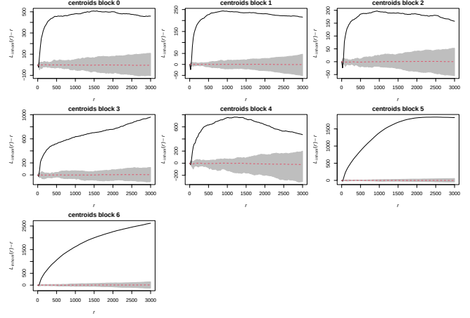
Figure 16: Independent spatstat confirmation: per-block inhomogeneous L_{\text{inhom}}(r) - r (observed, solid) vs the global-host-conditioned simulation envelope (shaded), for each of the seven super-site blocks, extended to r = 3\text{ km} . Observed lies above the envelope in every block, confirming residual aggregation beyond host that persists past 1 km.
