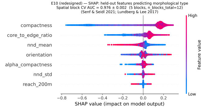
Figure 13: SHAP beeswarm plot for the held-out Random Forest (E10). Compactness is the dominant predictor; reach_200m (shape-independent connectivity) ranks last.
