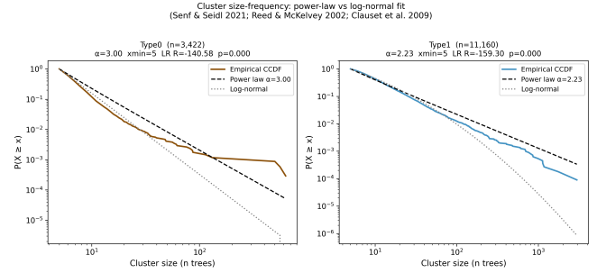
Figure 7: Complementary cumulative distribution functions (CCDF) of cluster size ( n ) per endpoint. Both are better described by a lognormal than a power law; Type 1 has the heavier upper tail, consistent with its larger mean cluster area.
