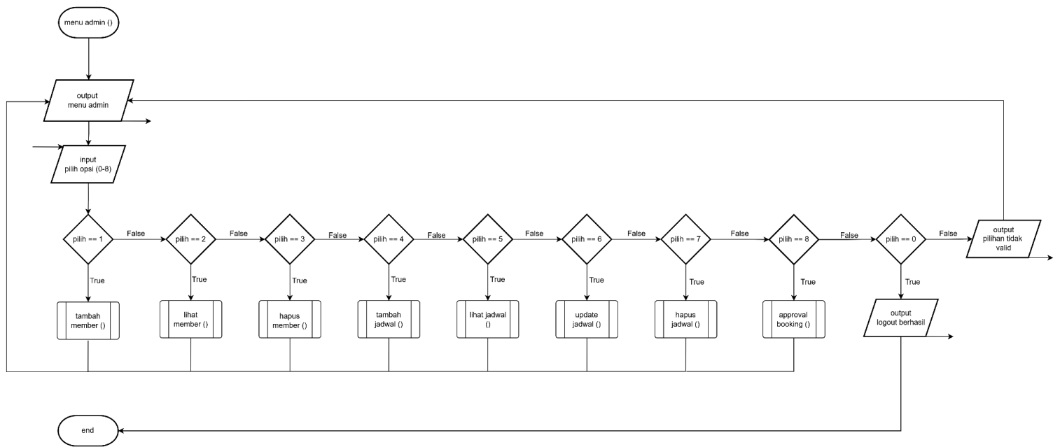
Gambar 2.4 Flowchart Menu Admin
