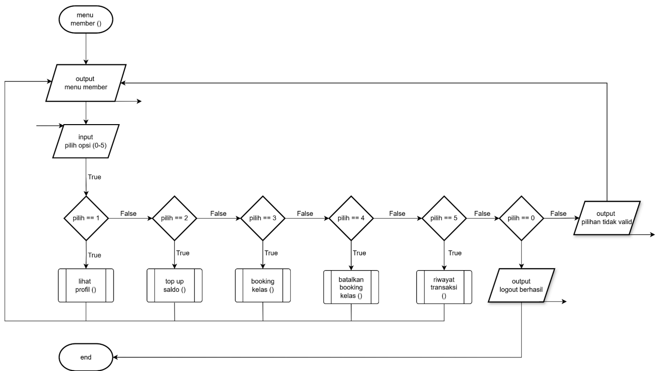
Gambar 2.14 Flowchart Menu User
