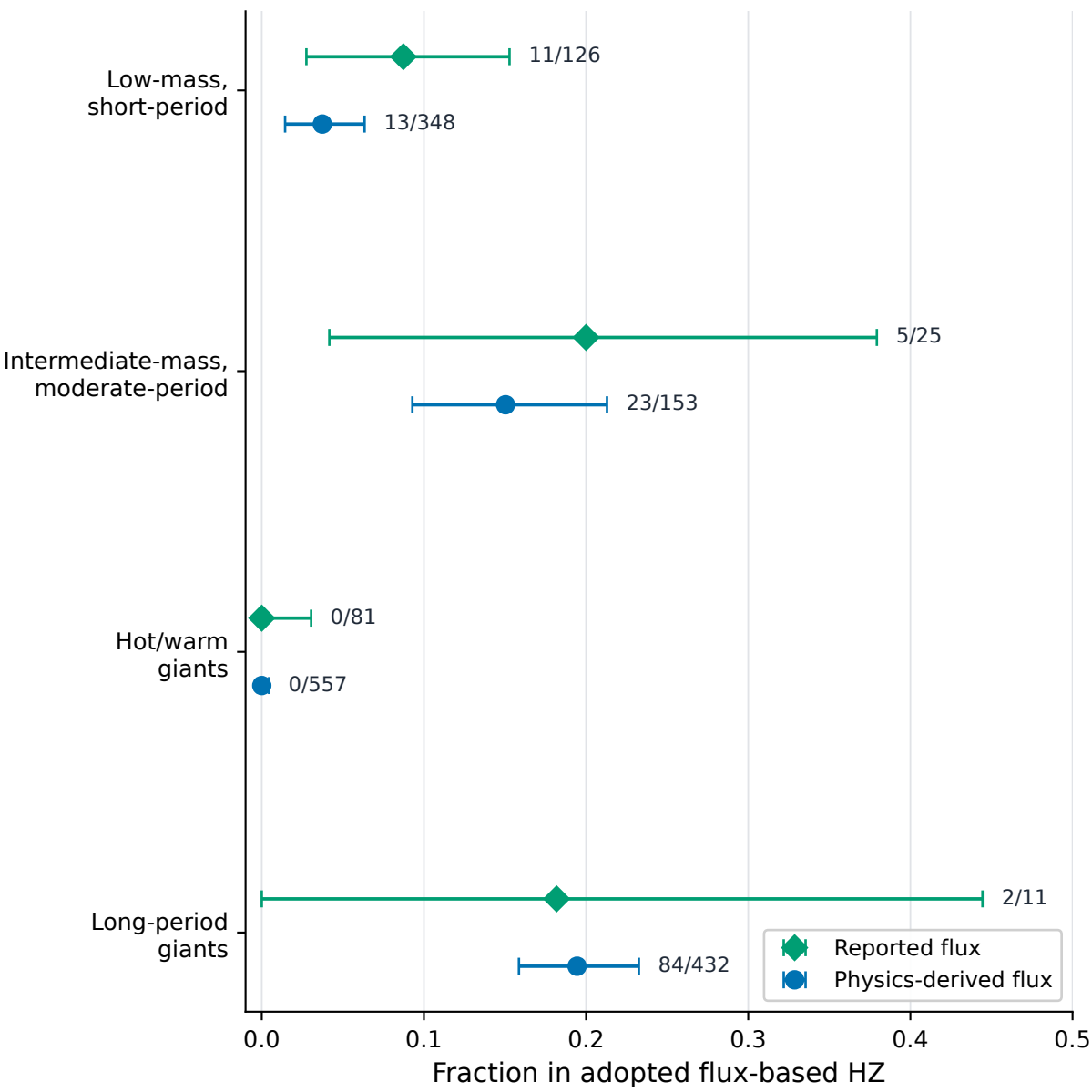
B. HZ overlap with 95% uncertainty
