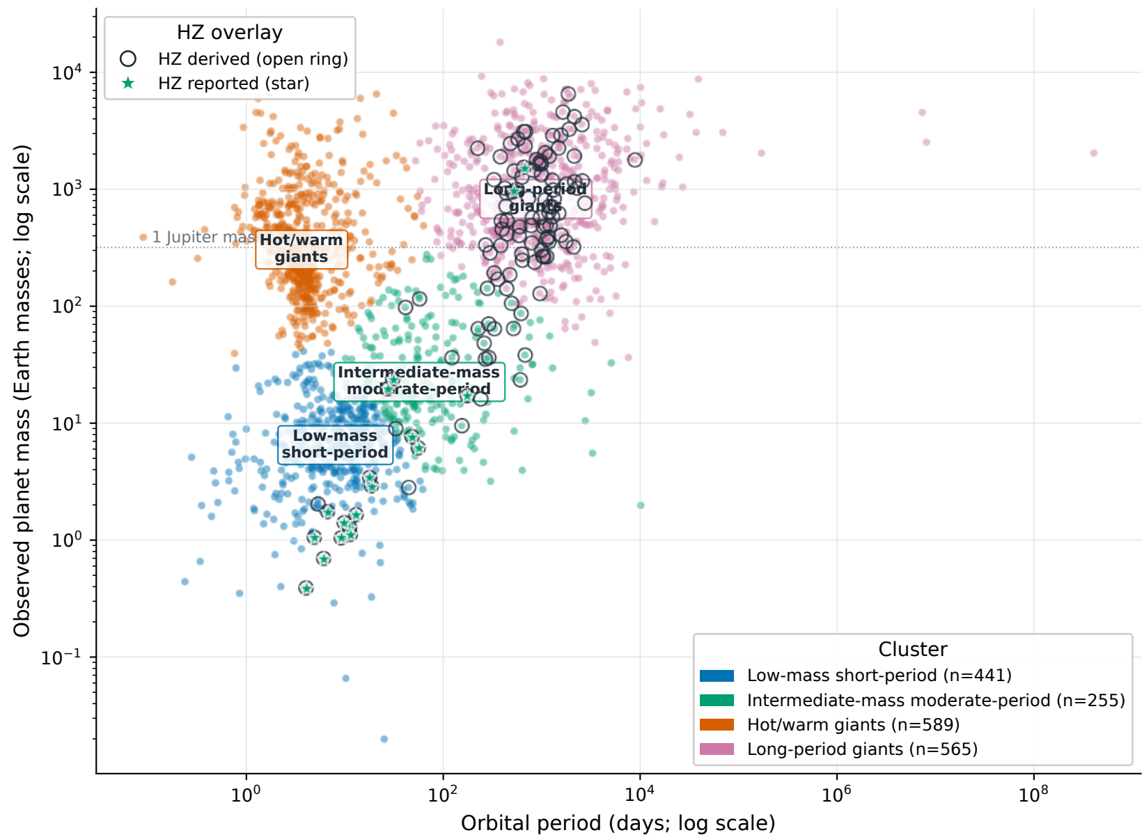
A. Four mass-period archetypes
