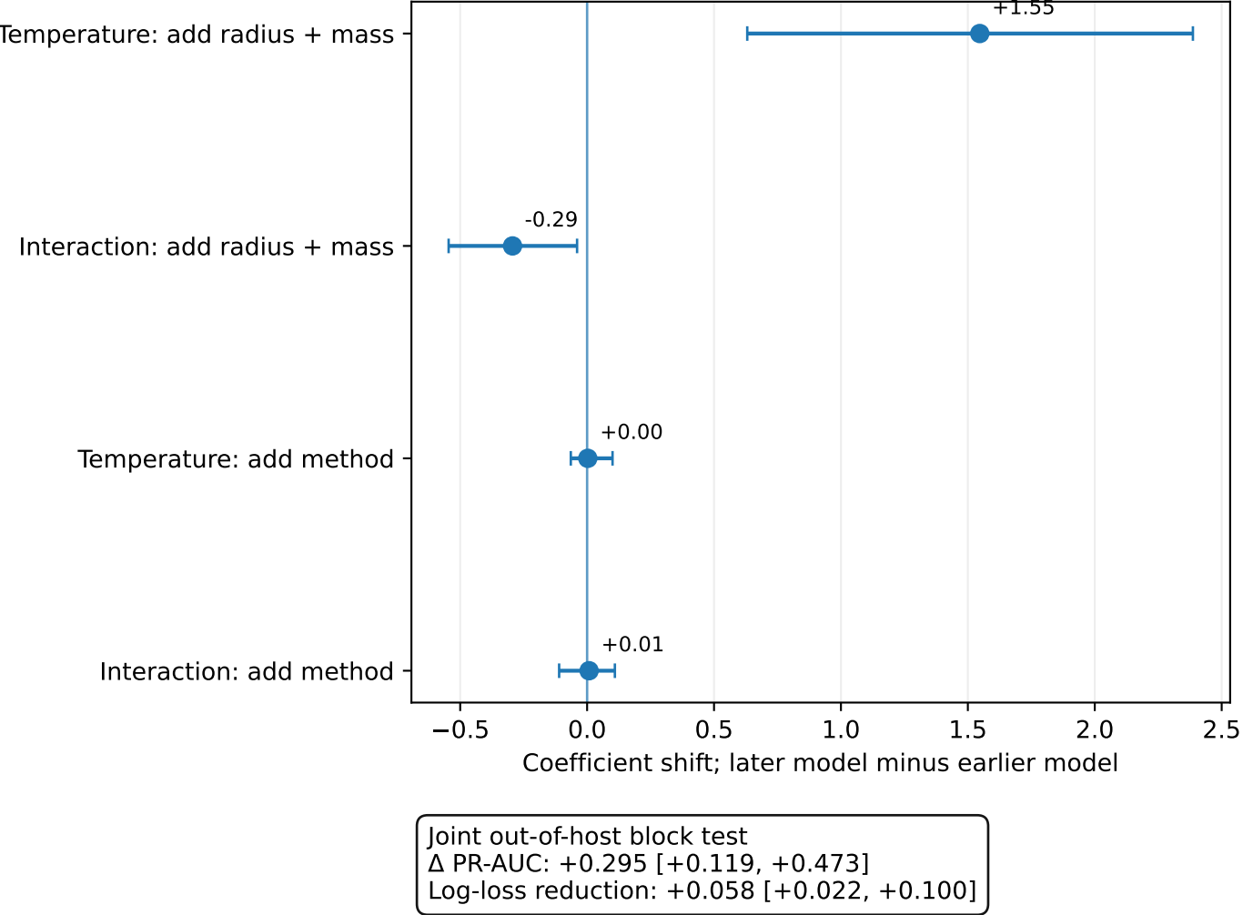
B. Paired coefficient shifts
