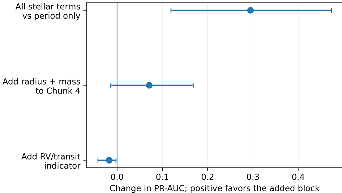
B. Incremental ranking value
