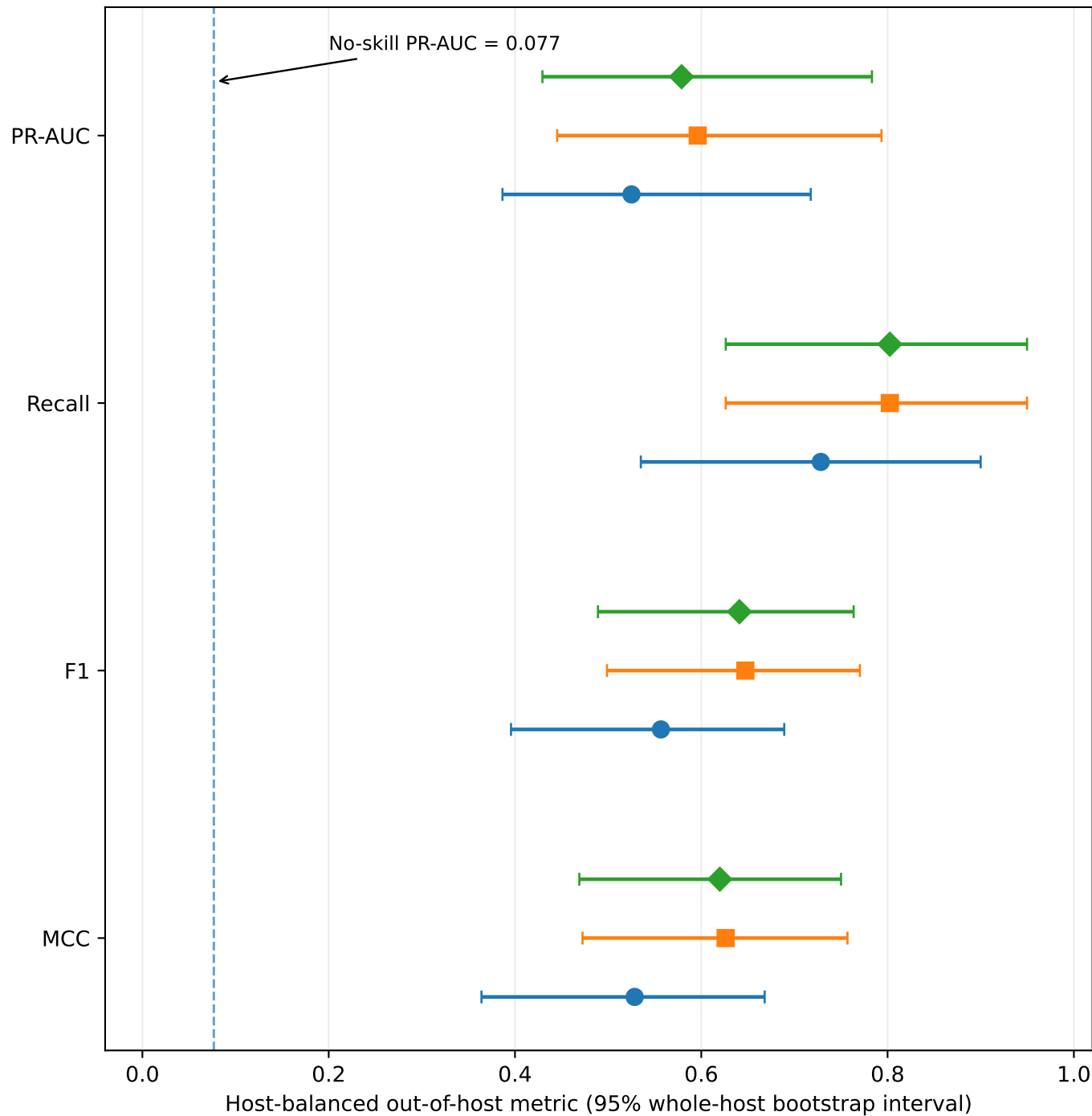
A. Controlled additions within one ridge-logistic family
