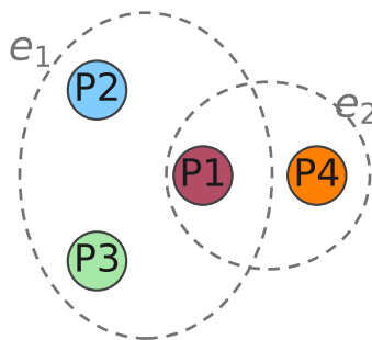
Hypergraph
