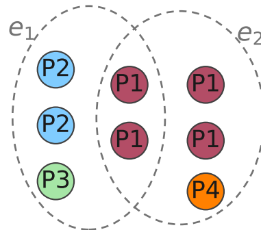
hb-graph
