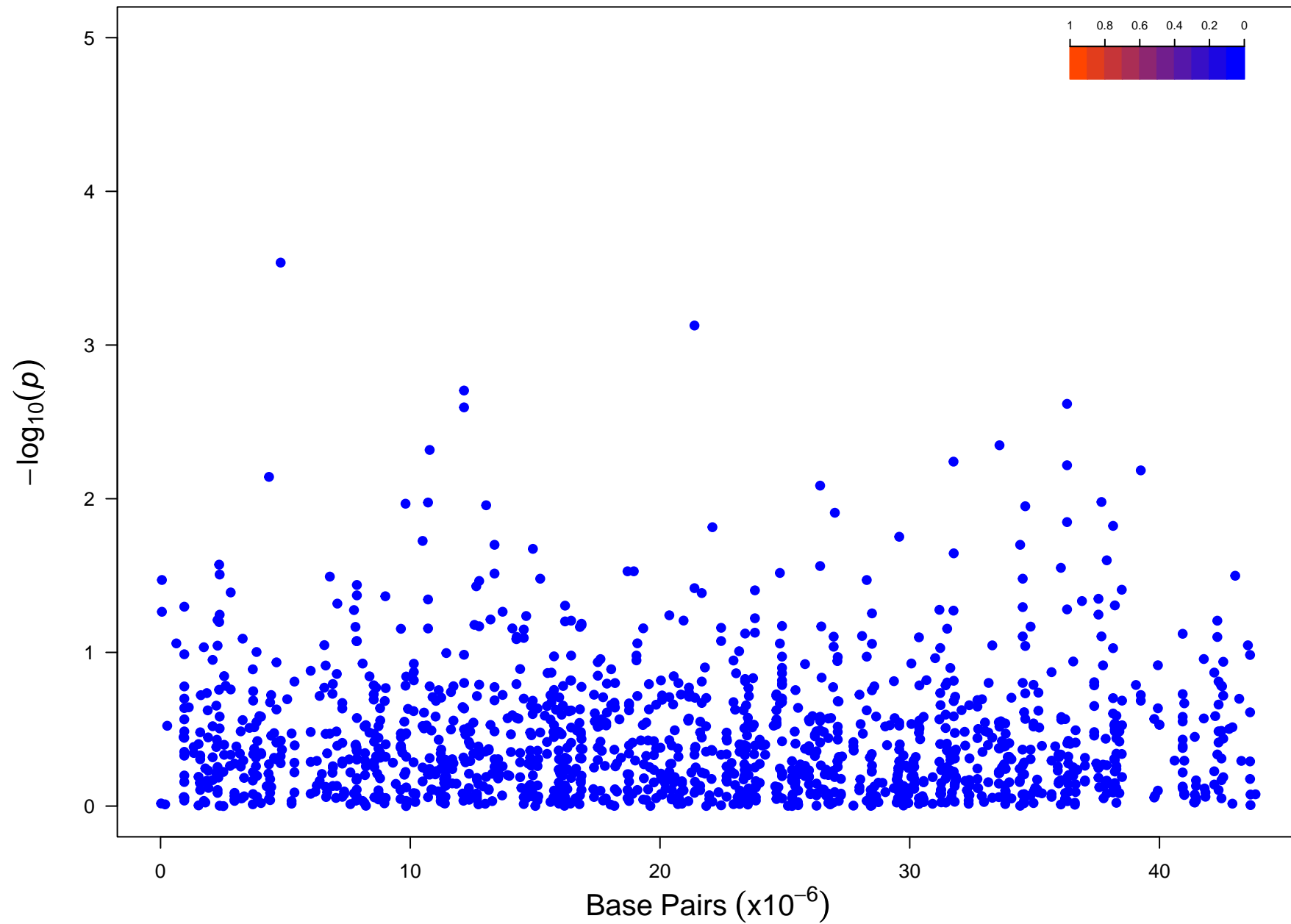
Chromosome 28
