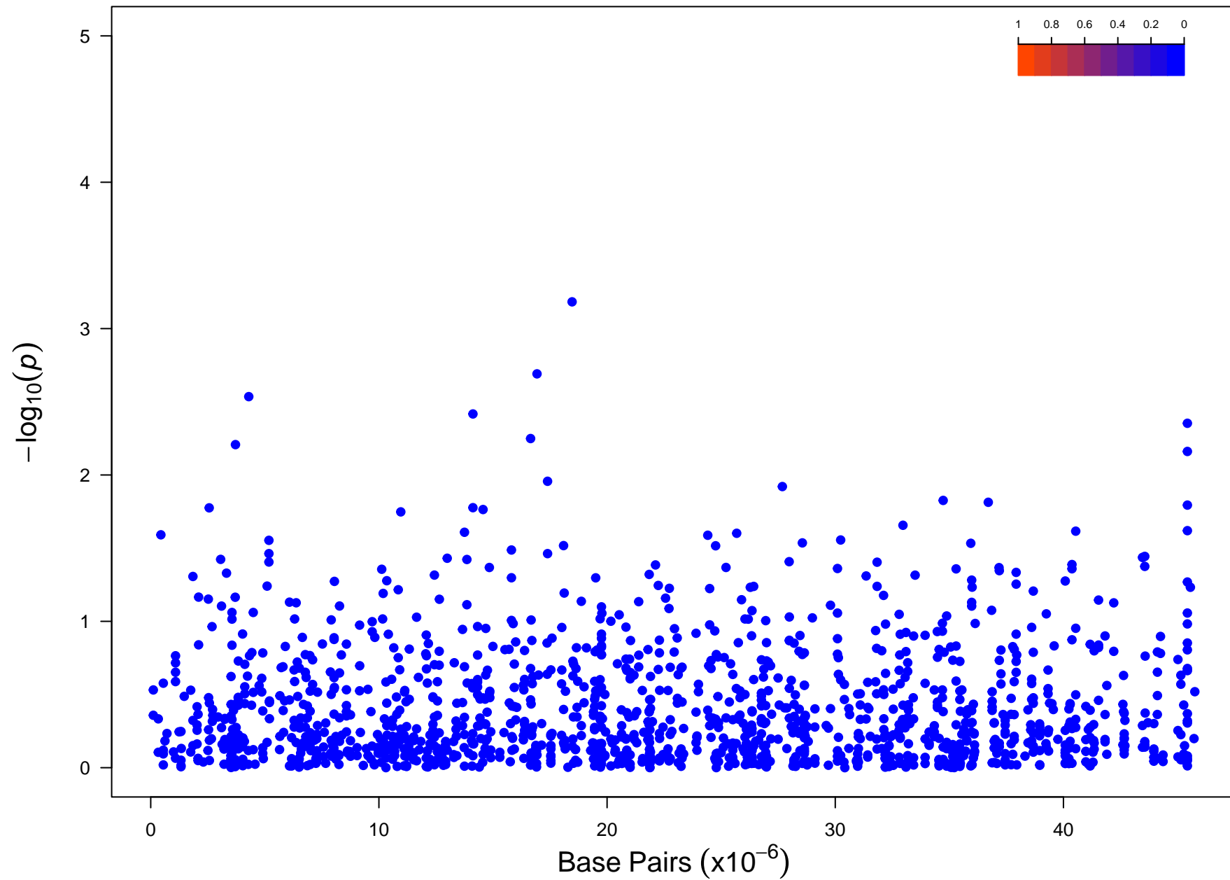
Chromosome 24
