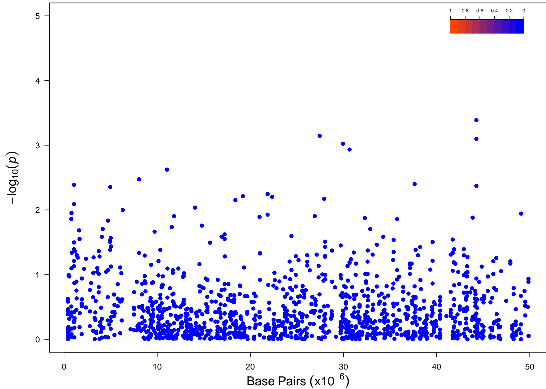
Chromosome 29
