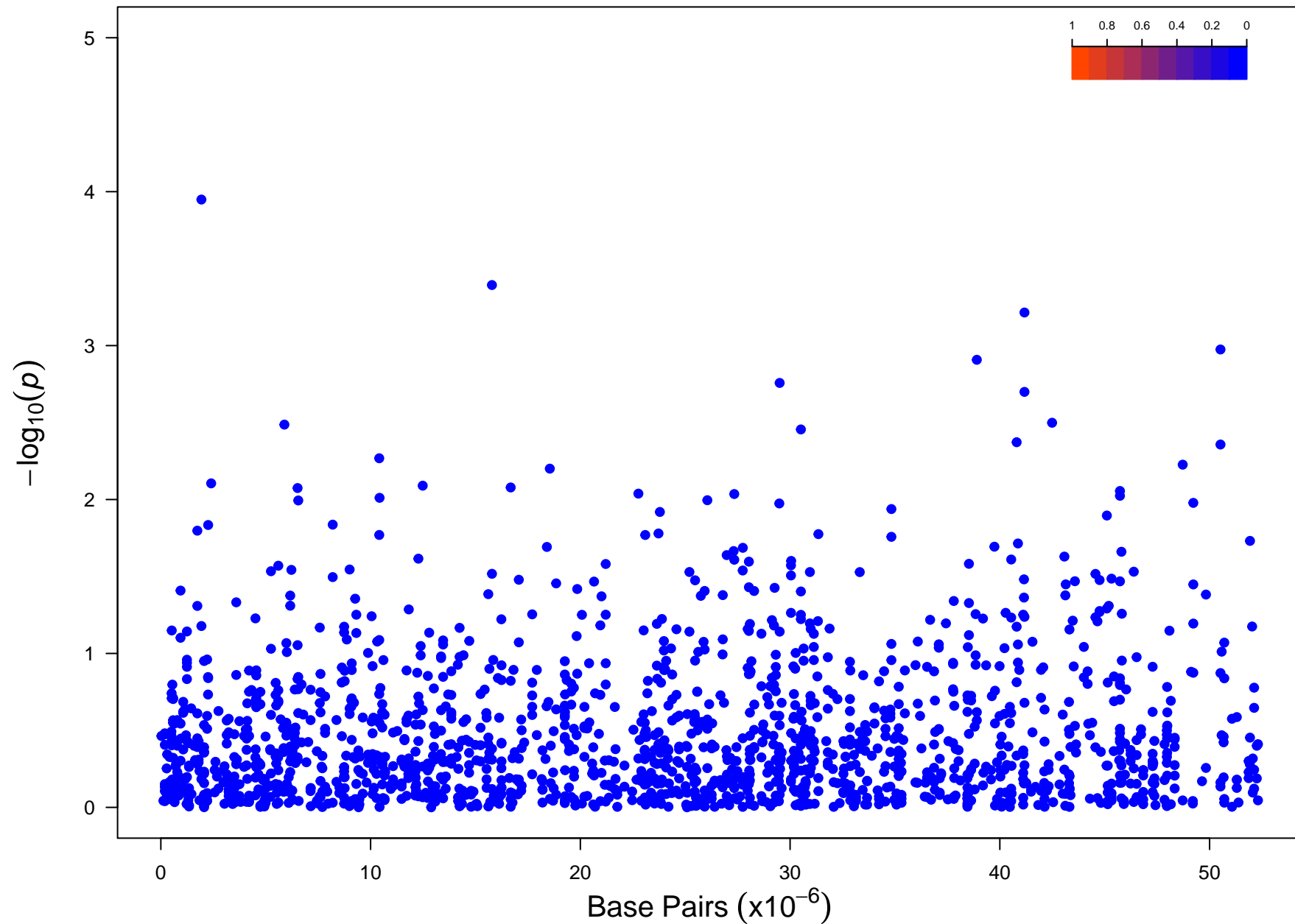
Chromosome 22
