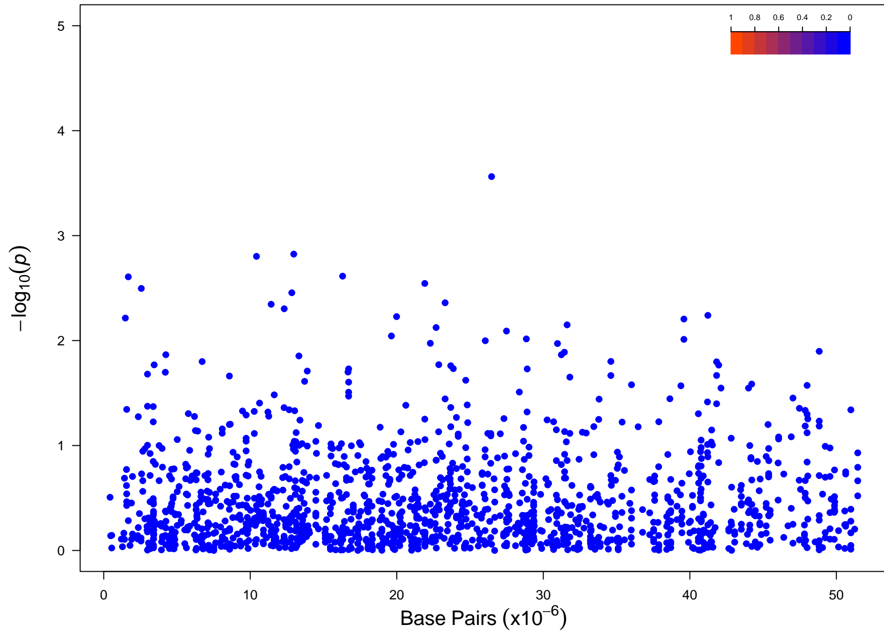
Chromosome 27
