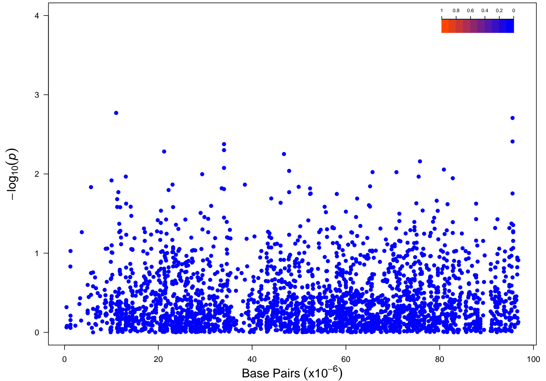
Chromosome 2
