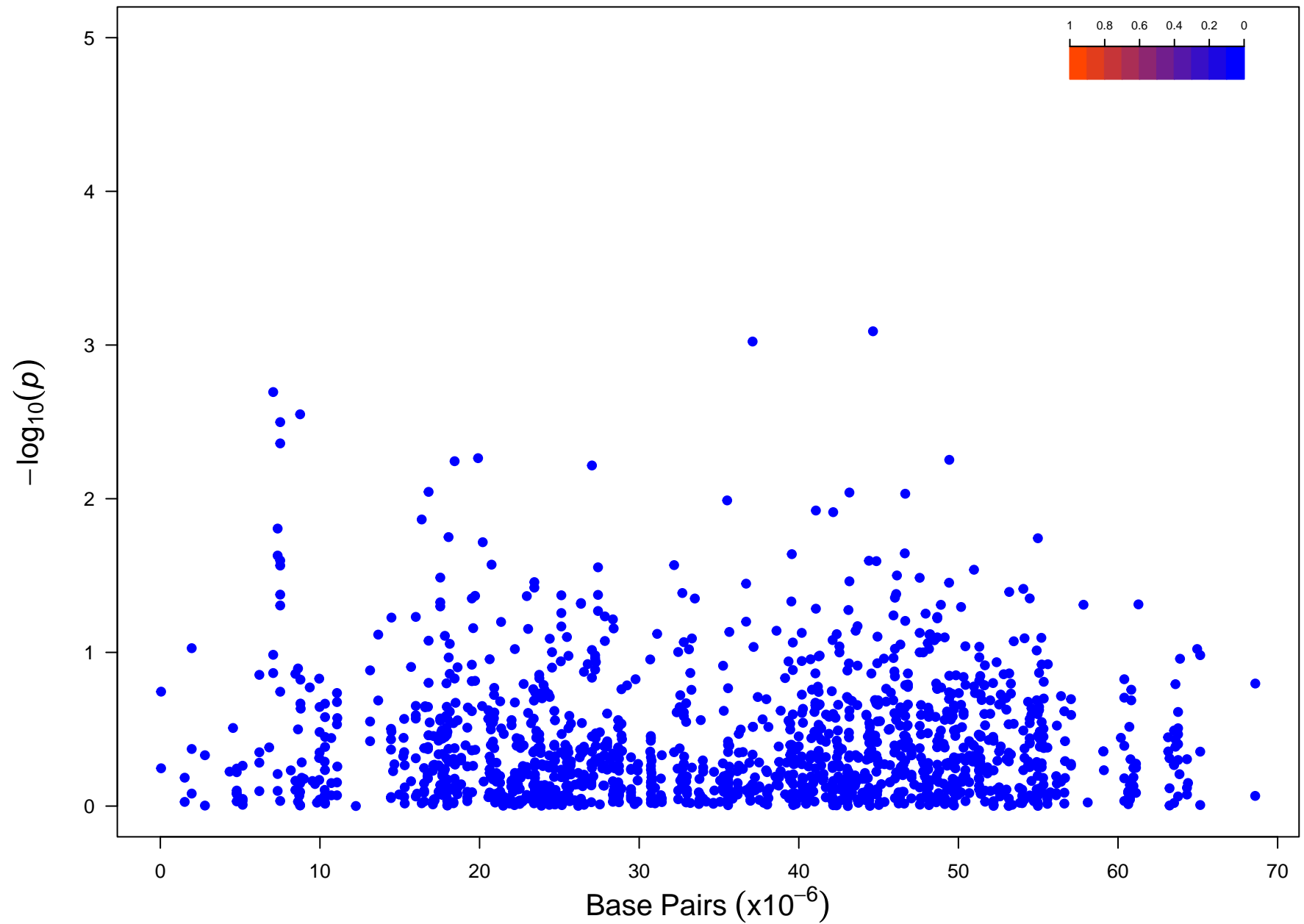
Chromosome 13
