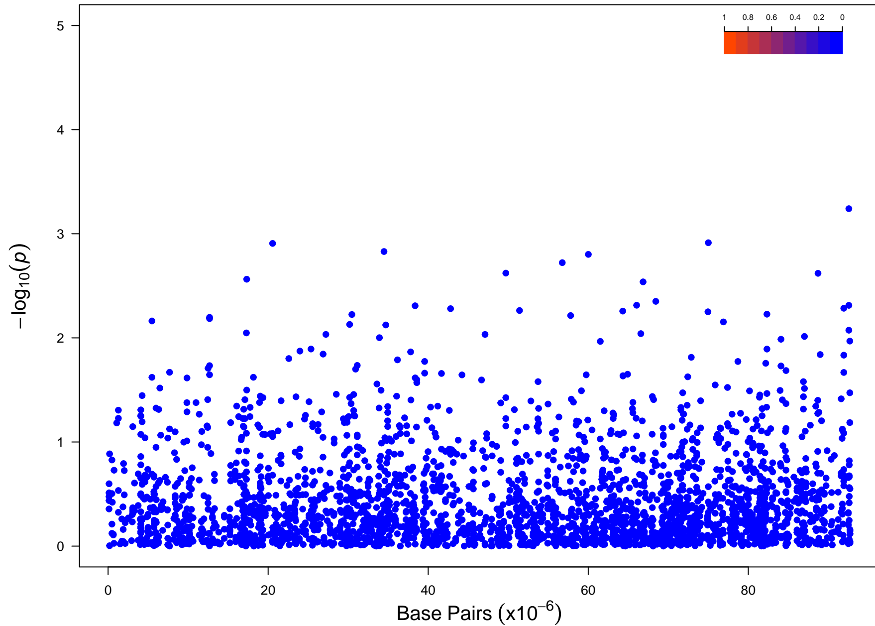
Chromosome 25
