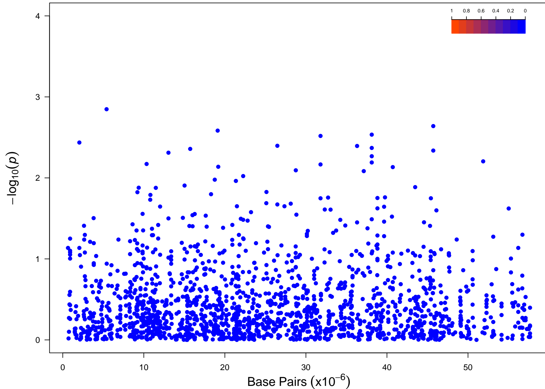
Chromosome 23
