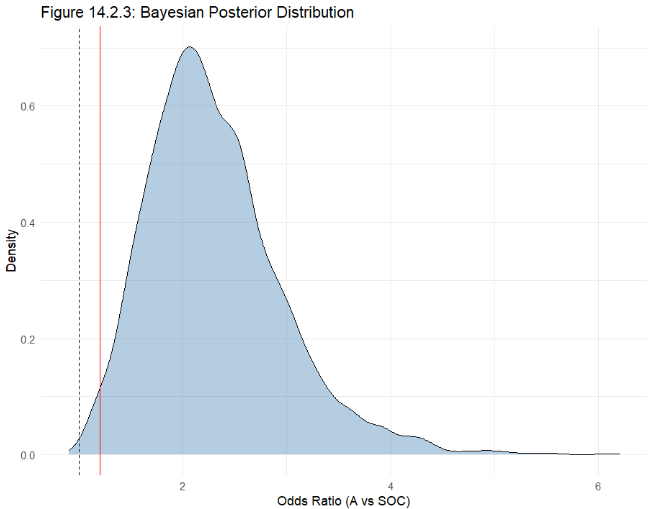
Figure 14.2.3: Bayesian Posterior Distribution of Treatment Effect
