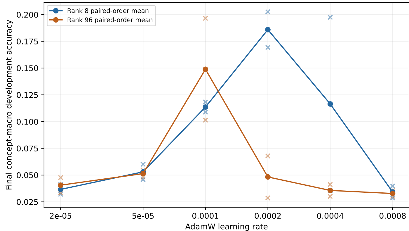
BANKING | Seed 2026 tuning grid | both orders retained
