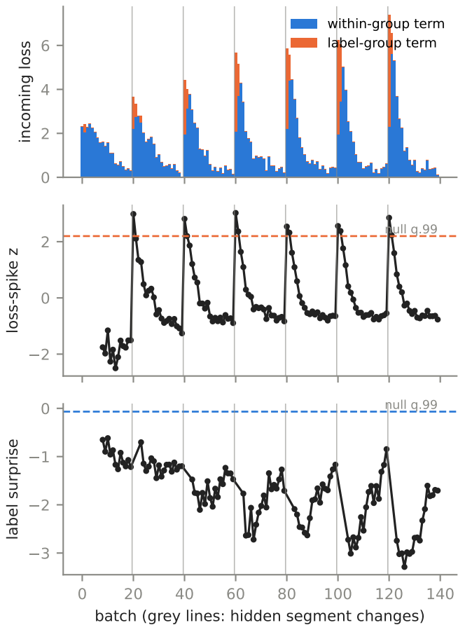
BANKING77, class-incremental
