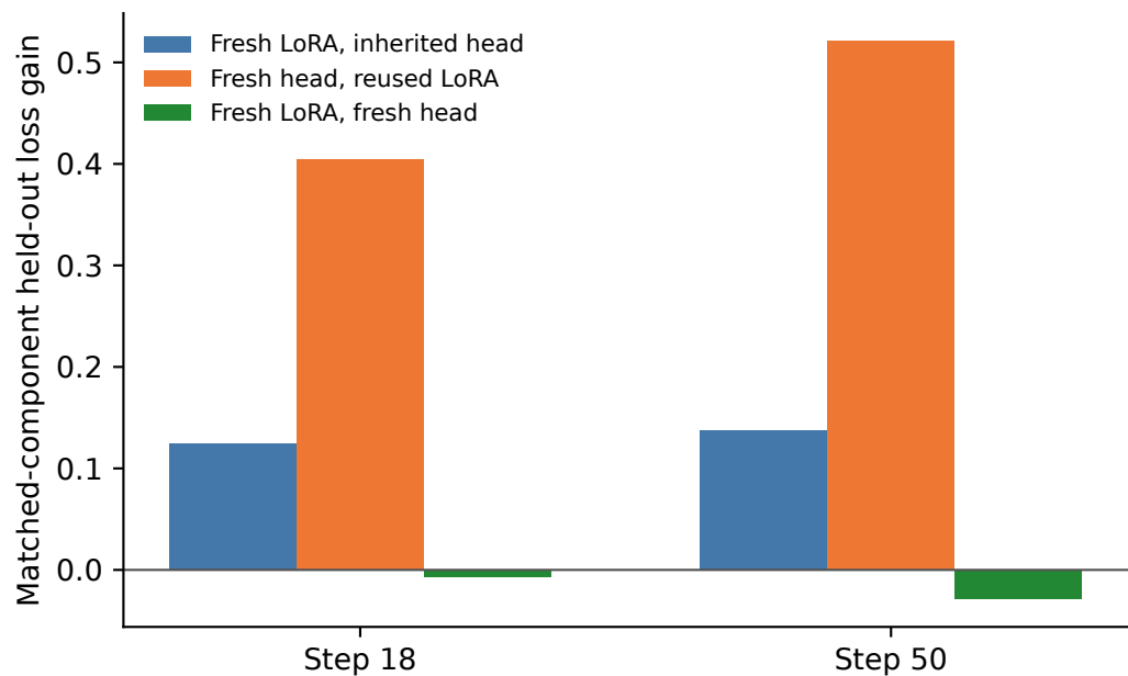
Classifier reset is a substantial factor
