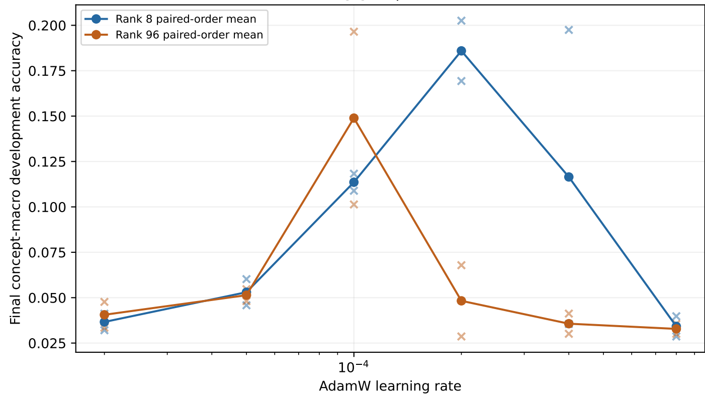
Seed 2026 tuning grid | both orders retained
