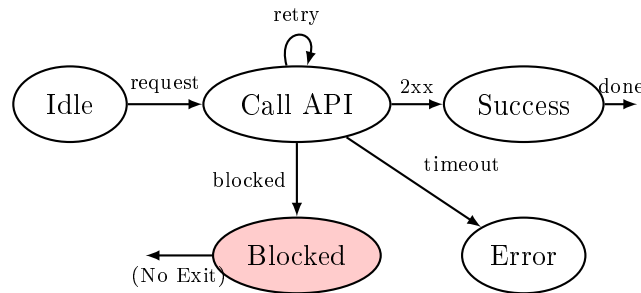
Figure 11: Agentic automaton. Without EXIT and observable error codes, agent loops indefinitely, times out, or escalates incorrectly.
