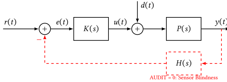
Figure 4: Open-loop failure mode. When AUDIT fails ( H = 0 ), the feedback path is severed. Equivalent failure occurs if GOVERN ( K = 0 ) or EXIT ( e(t) \equiv 0 ) is removed.
