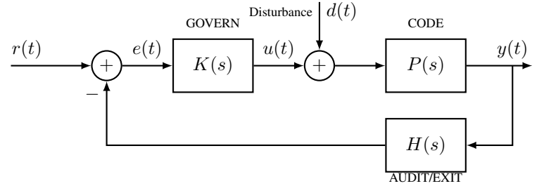
Fig. 9: Control-theoretic model of corrigible infrastructure. K(s) : governance controller. H(s) : sensor/audit function. P(s) : plant (infrastructure). d(t) : environmental disturbance.
