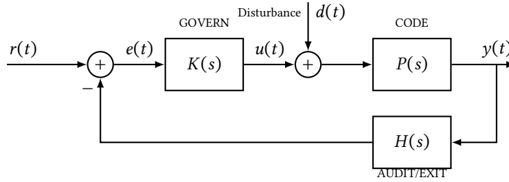
Figure 6: Control-theoretic model of corrigible infrastructure. K(s) : governance controller. H(s) : sensor/audit function. P(s) : plant (infrastructure). d(t) : environmental disturbance.
