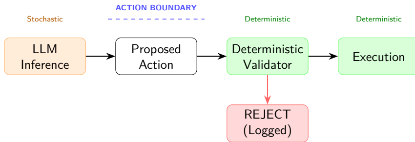
Figure 3: Action Boundary Protocol. Probabilistic inference (orange) produces proposed actions. A deterministic validator (green) enforces hard constraints before execution. Invalid actions are rejected and logged. The action boundary separates epistemic generation from authorized execution.
