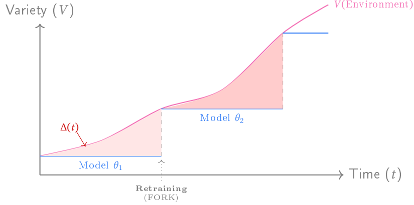
Figure 3: The Temporal Variety Gap. Environmental variety V(e) evolves continuously (curve). A fixed model \theta (stepped line) diverges from reality. The shaded area represents accumulated error. Only FORK rights allow the gap to be closed via retraining.
