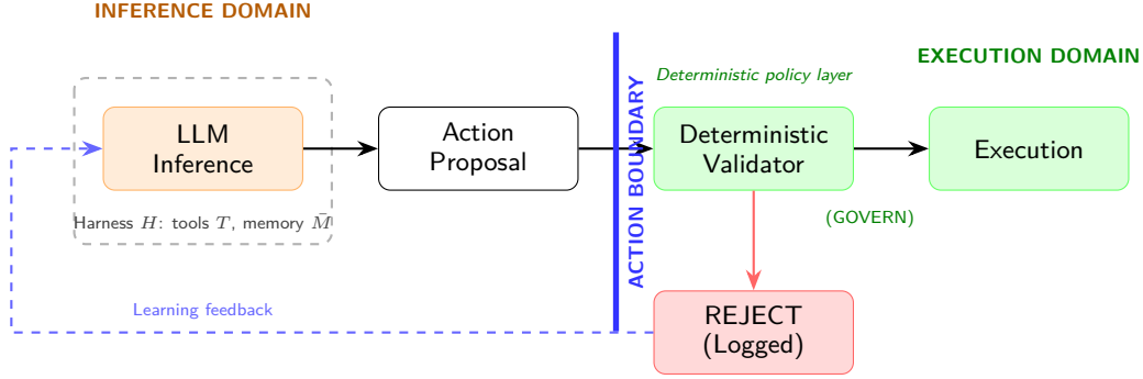
Figure 4: Action Boundary Protocol. Probabilistic inference (orange) produces action proposals from within its harness envelope (orchestration, tools T , persistent memory M ): internal delegation, however deep or wide, is invisible to the validator, which receives only typed proposals. The deterministic policy layer (green, implementing GOVERN) enforces hard constraints before execution. Invalid actions are rejected, logged, and fed back for learning. The vertical Action Boundary separates the inference domain from the execution domain: the architectural instantiation of corrigibility in agentic systems.
