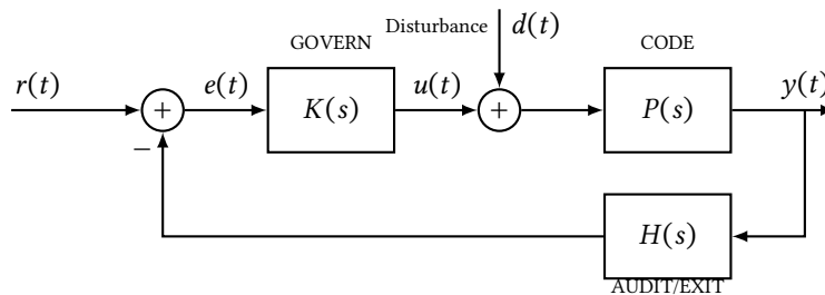
Figure 3: Control-theoretic model of corrigible infrastructure. K(s) : governance controller. H(s) : sensor/audit function. P(s) : plant (infrastructure). d(t) : environmental disturbance.
