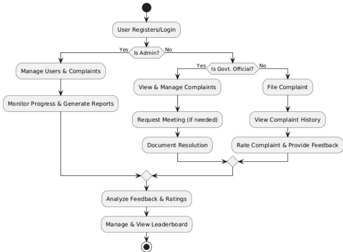
Figure 4.2: Activity Diagram
