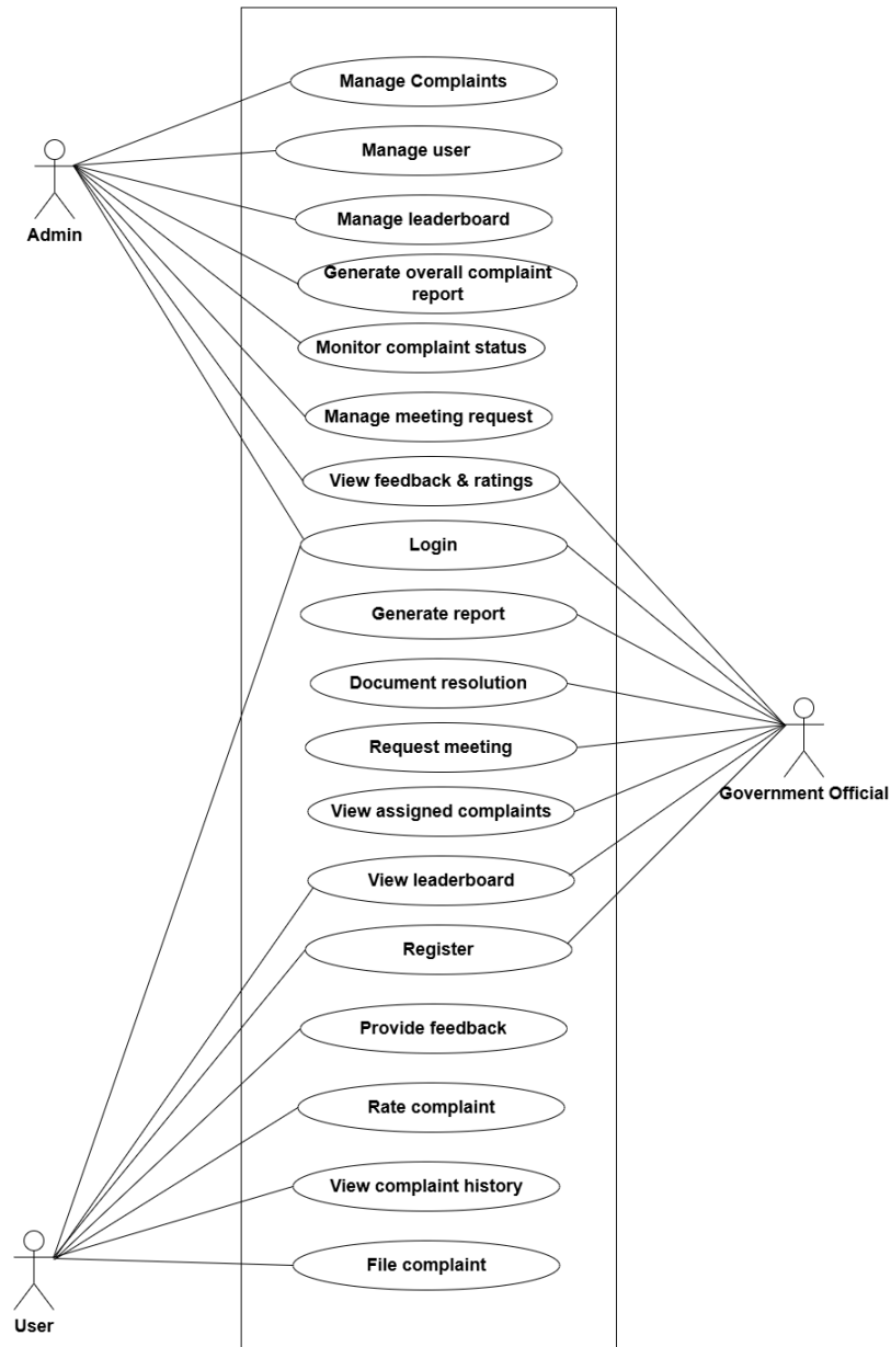
Figure 4.1: Use Case Diagram
