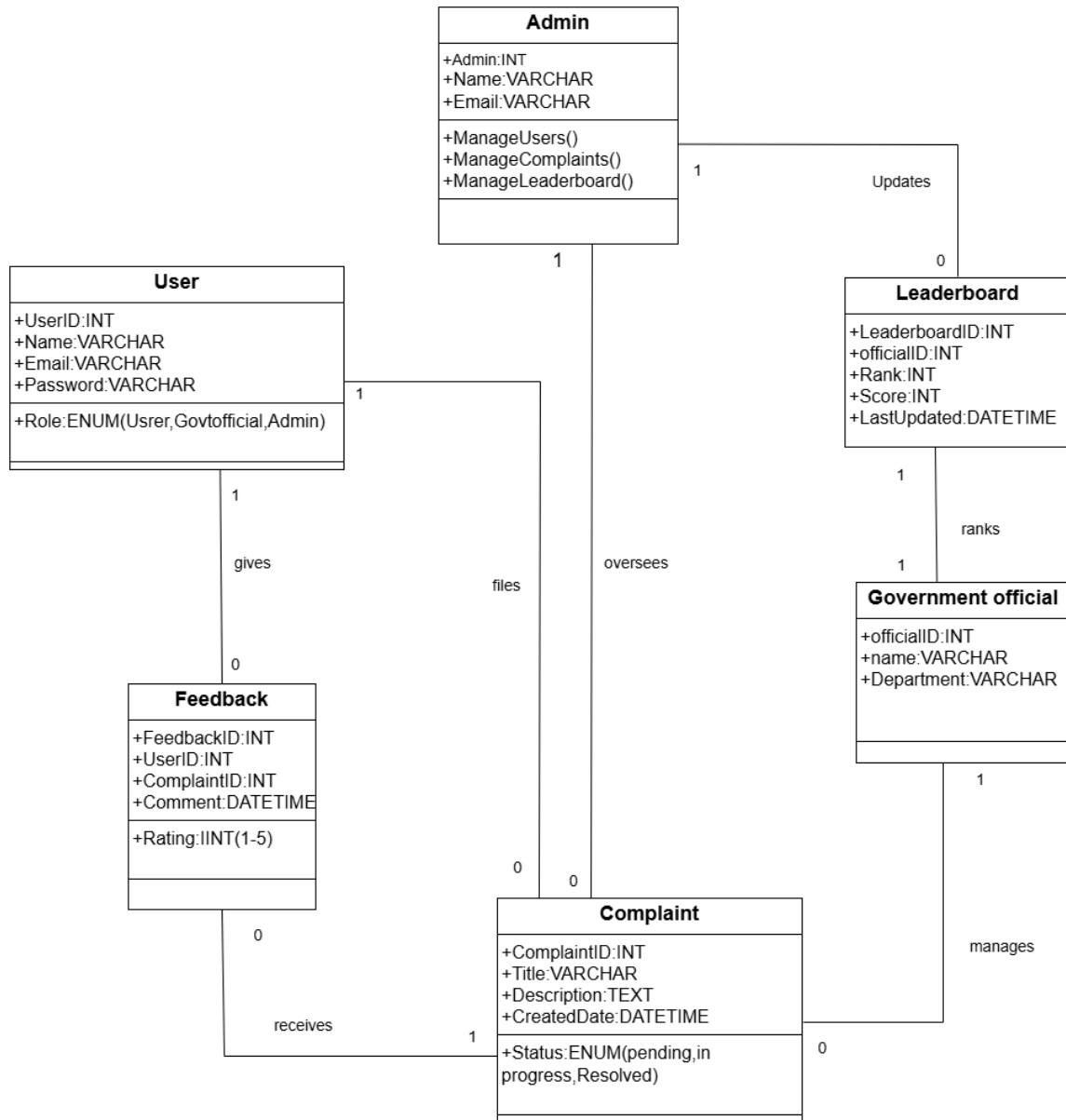
Figure 4.3: Class Diagram
