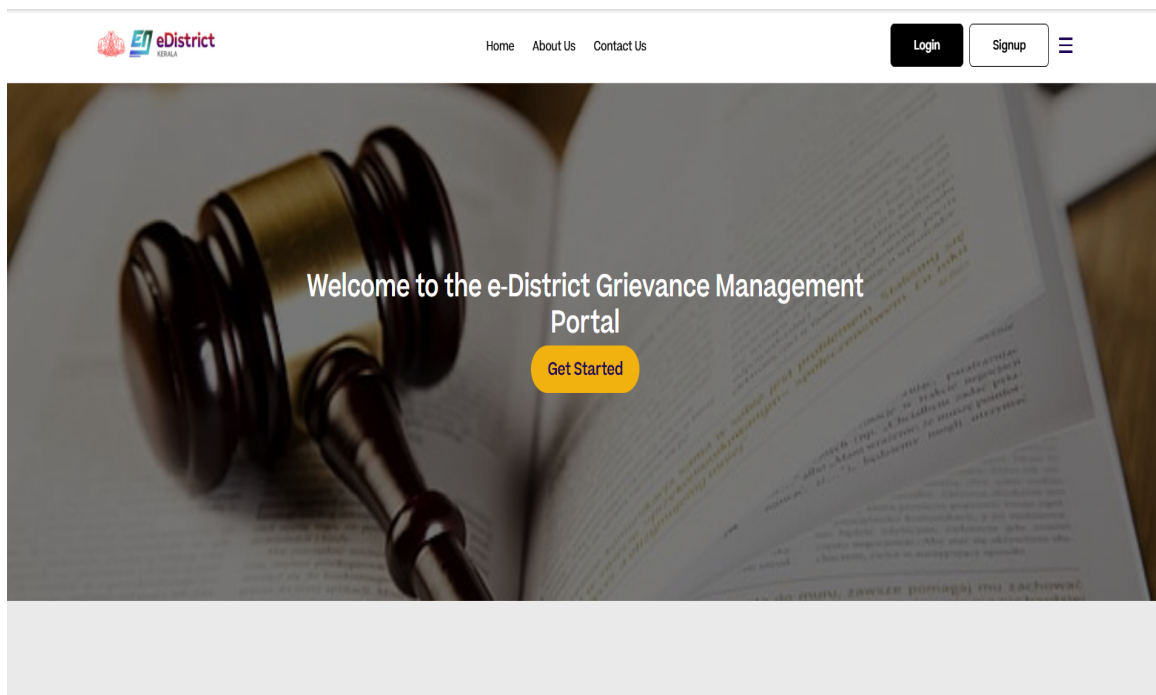
Home Page
