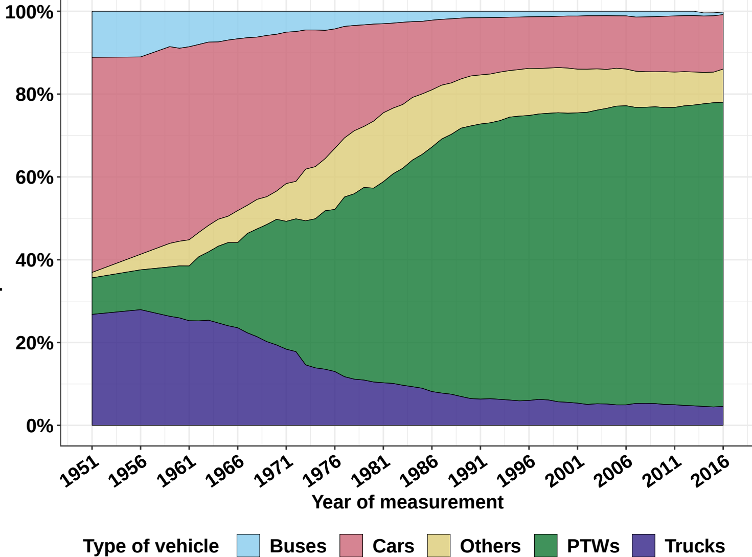
Vehicle composition of the traffic stream
