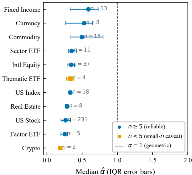
Shape parameter \hat{\alpha} by asset class (identified subset, n = 352 ; VIX excluded)
