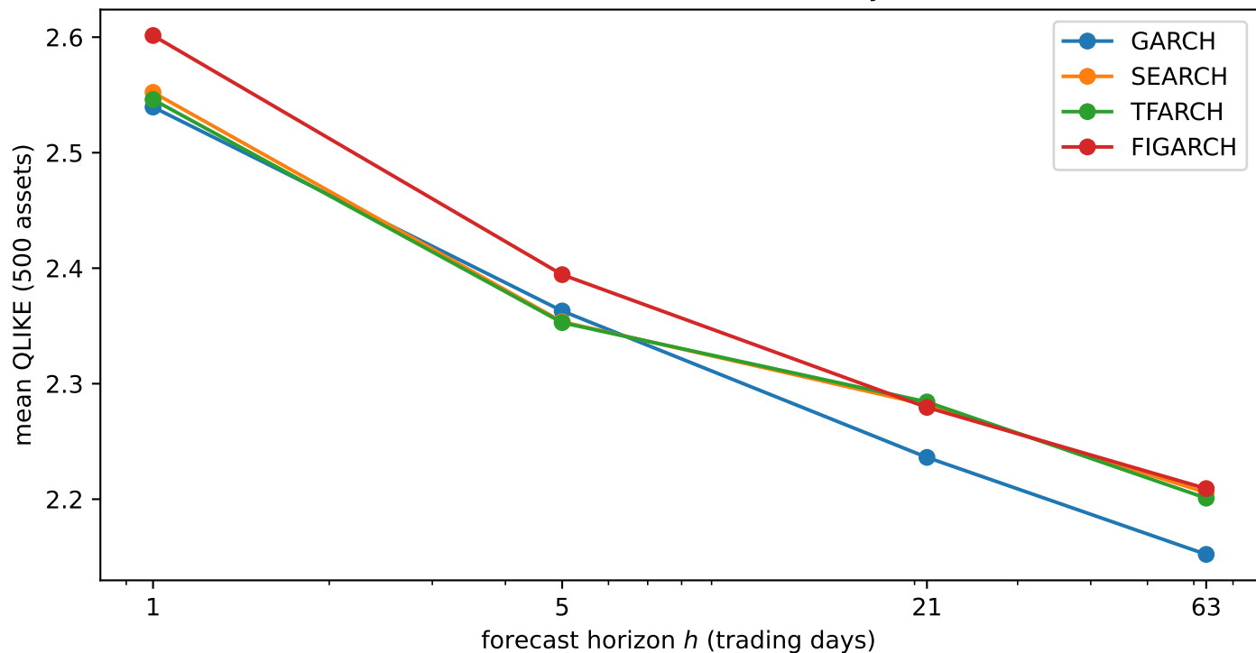
Out-of-sample QLIKE by horizon (75% MCS: all four at h=1,5 ; GARCH only at h=21,63 )
