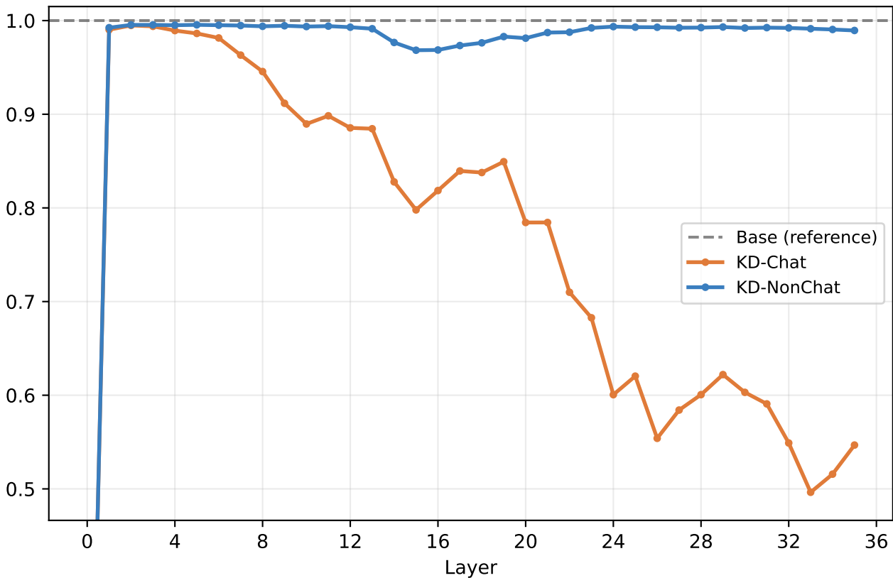
Cosine Similarity to Base Refusal Direction
