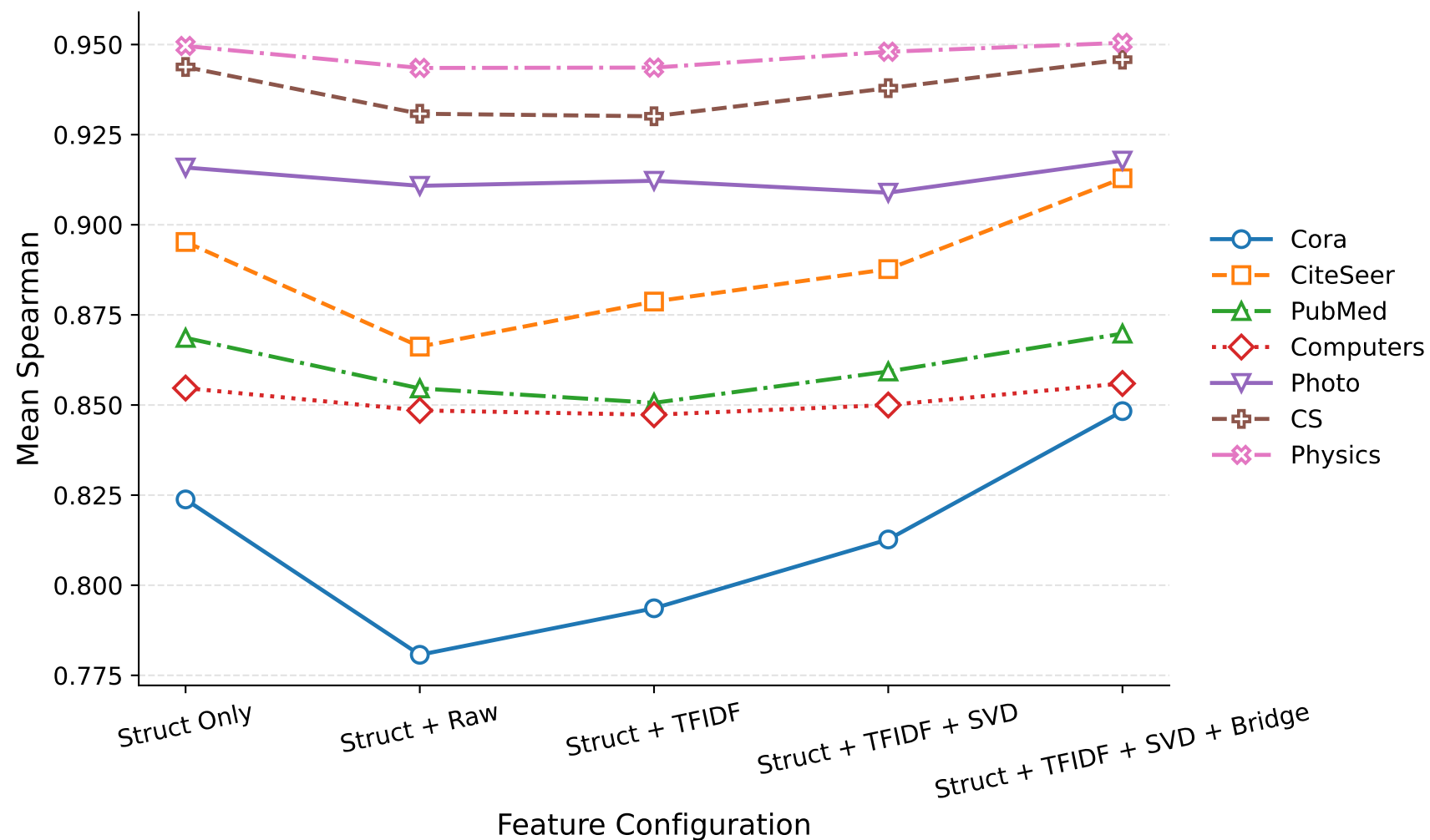
Structural-Semantic Ablation Comparison
