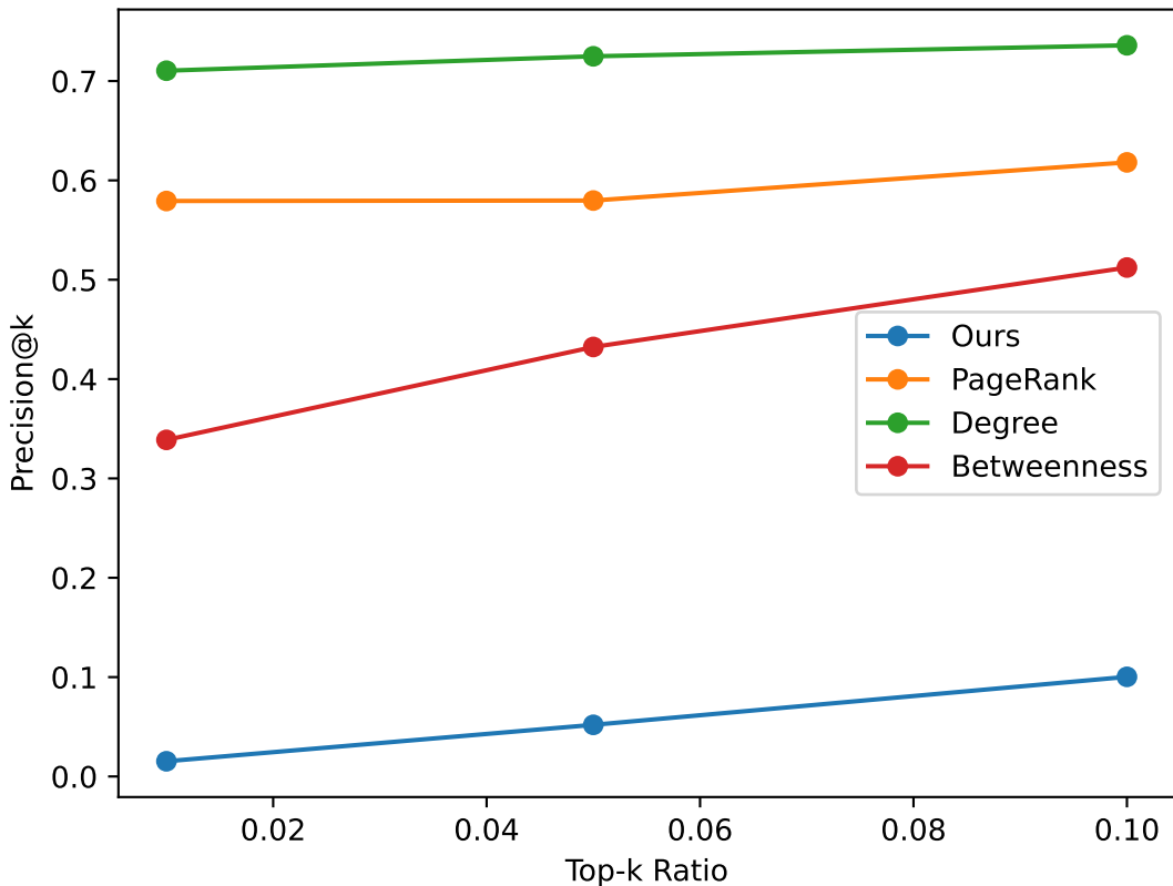
CS Top-k Precision
