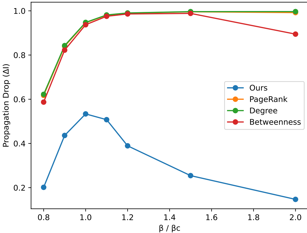
CS Robustness
