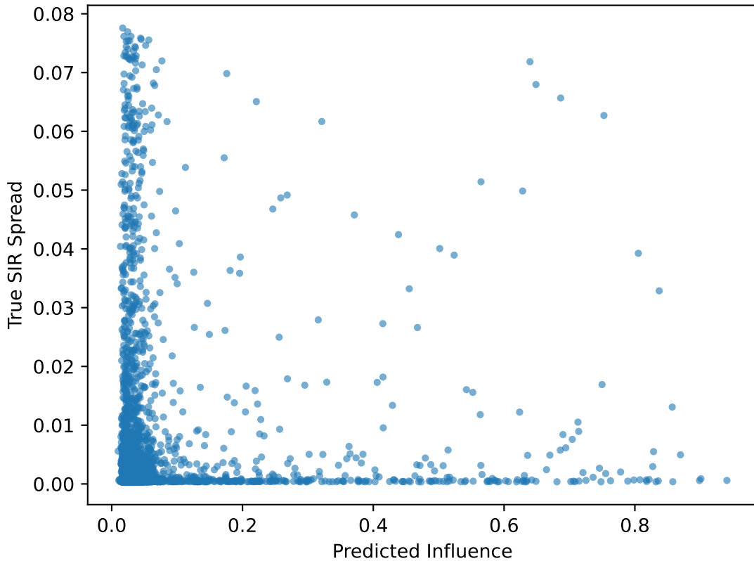
CiteSeer Spread Prediction
