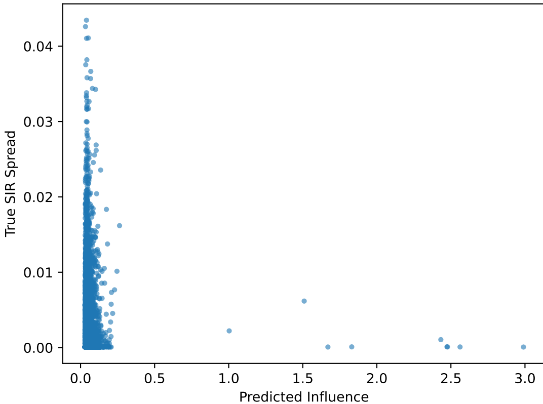
Computers Spread Prediction
