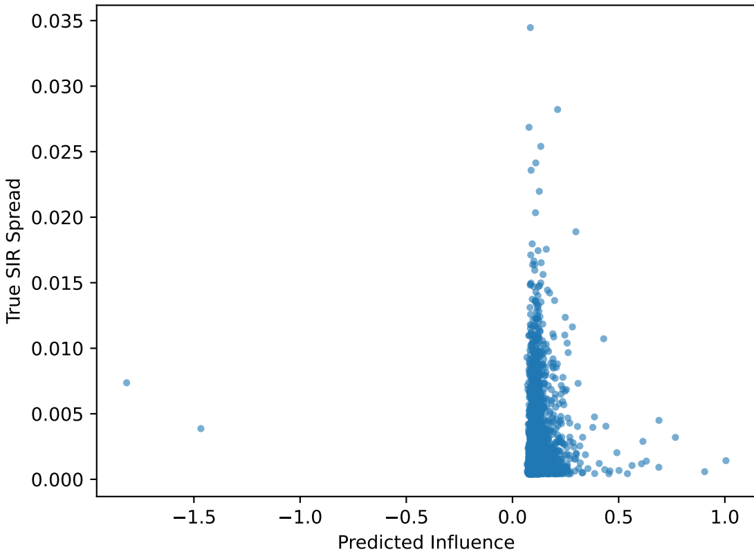
Cora Spread Prediction
