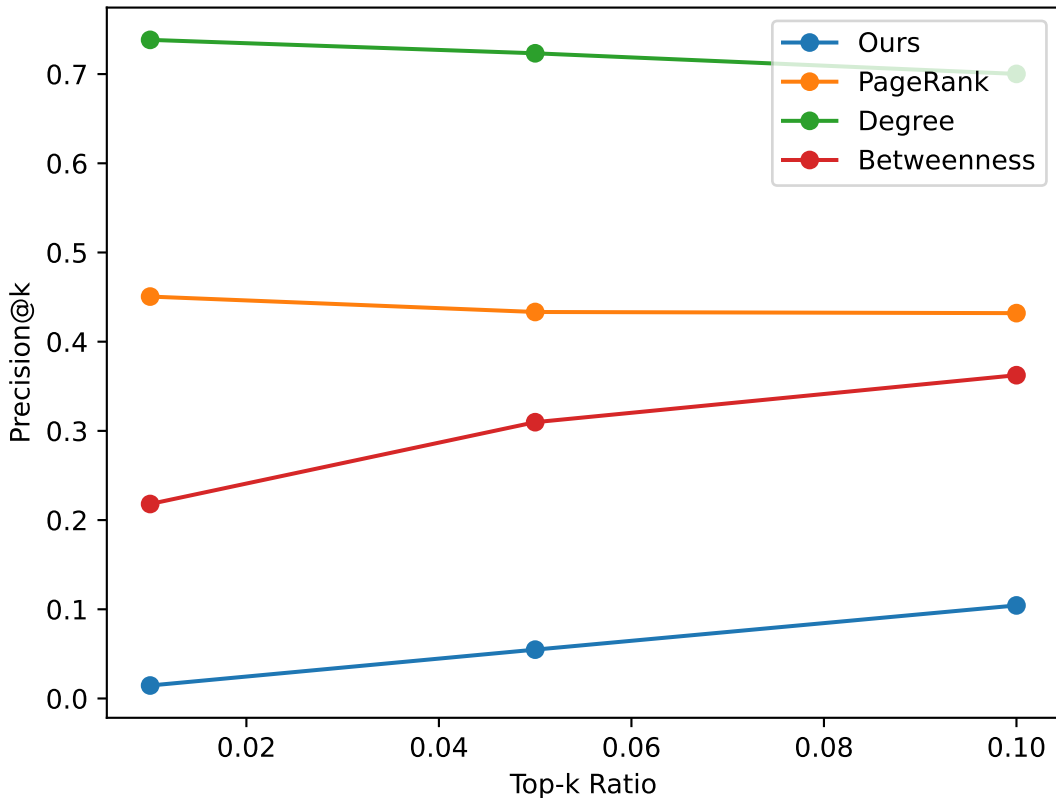
Physics Top-k Precision
