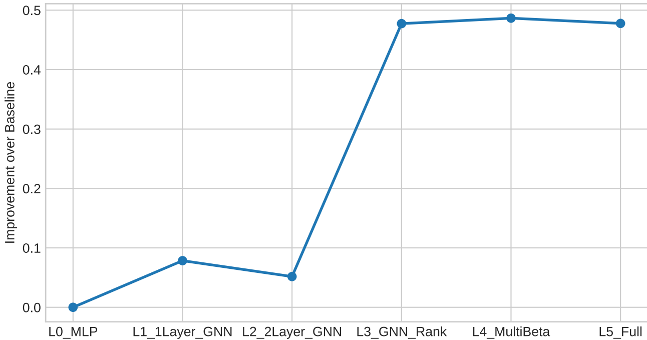
Performance Gain over Baseline
