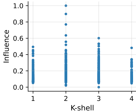
K-shell \rho=0.06
