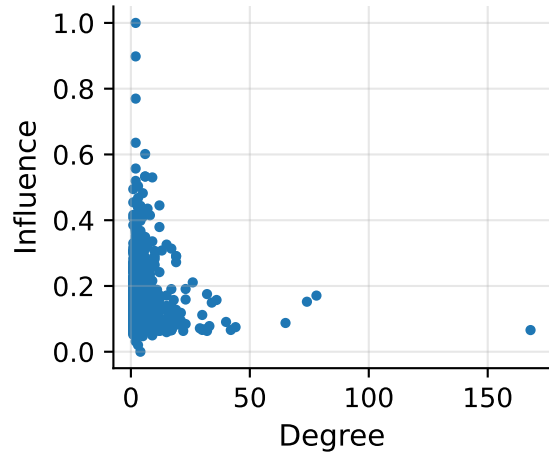
Degree \rho=0.07
