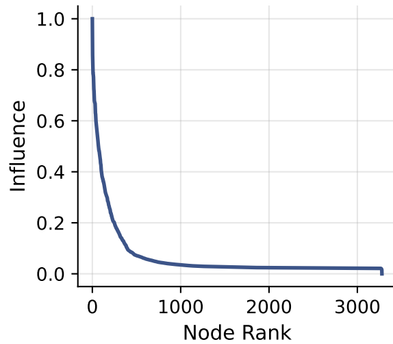
(e) Influence Ranking
