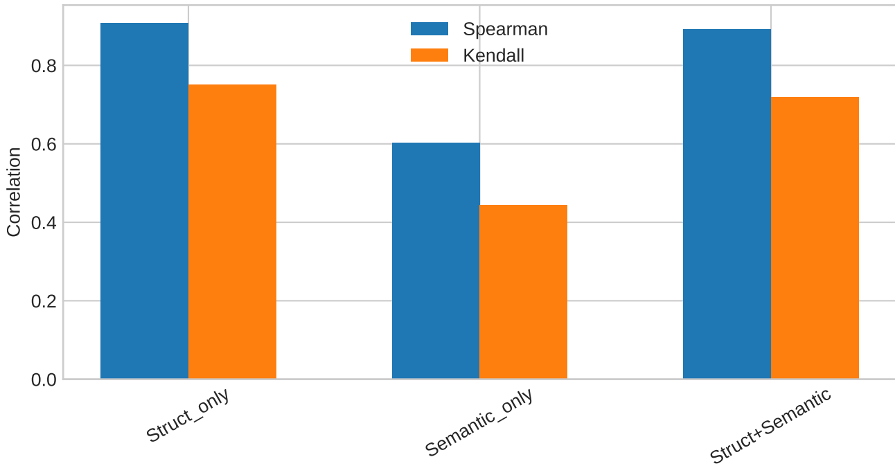
CiteSeer Ablation Study
