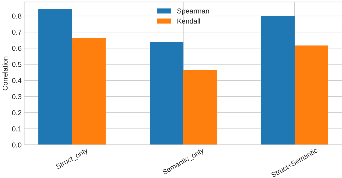
Cora Ablation Study
