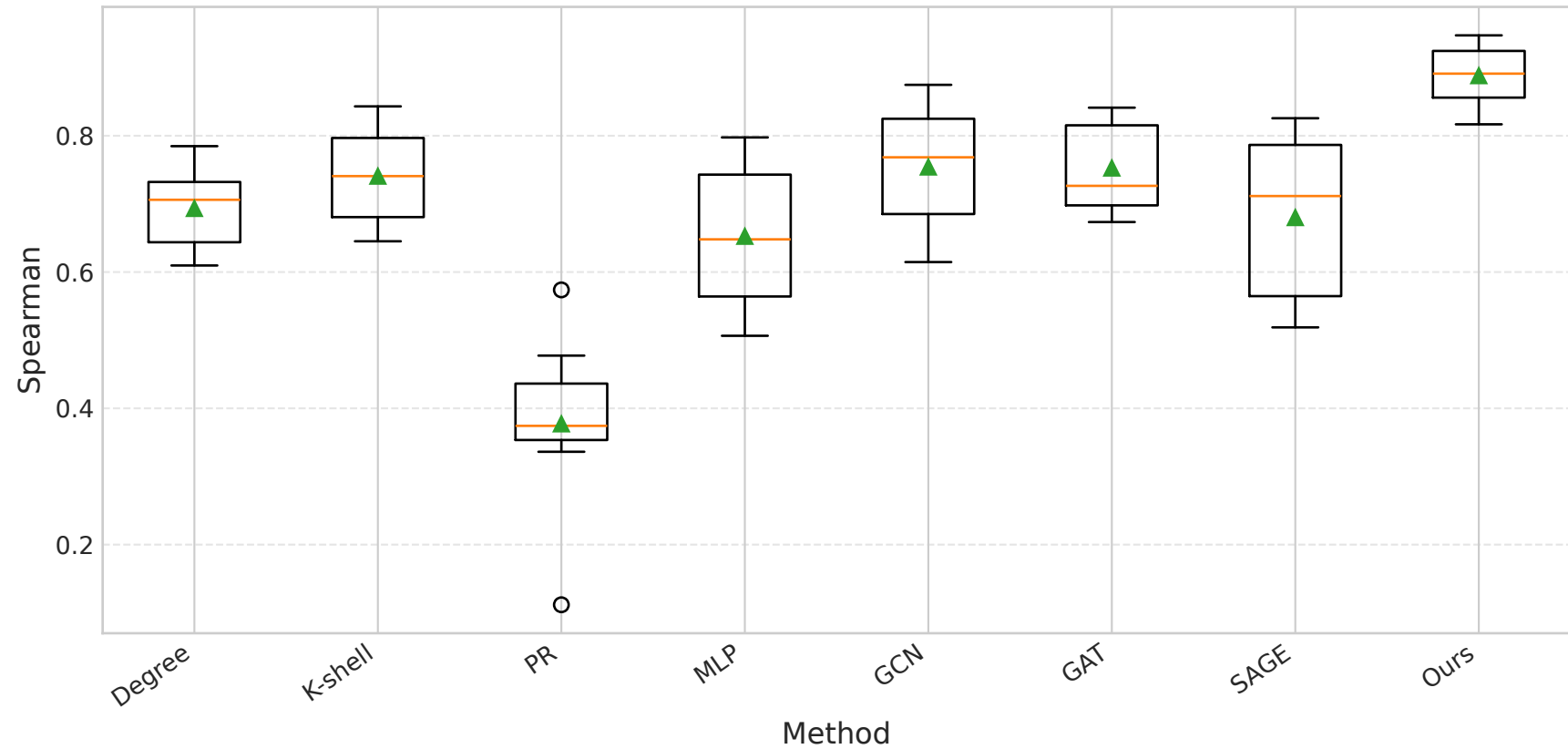
Distribution of Spearman Across Datasets
