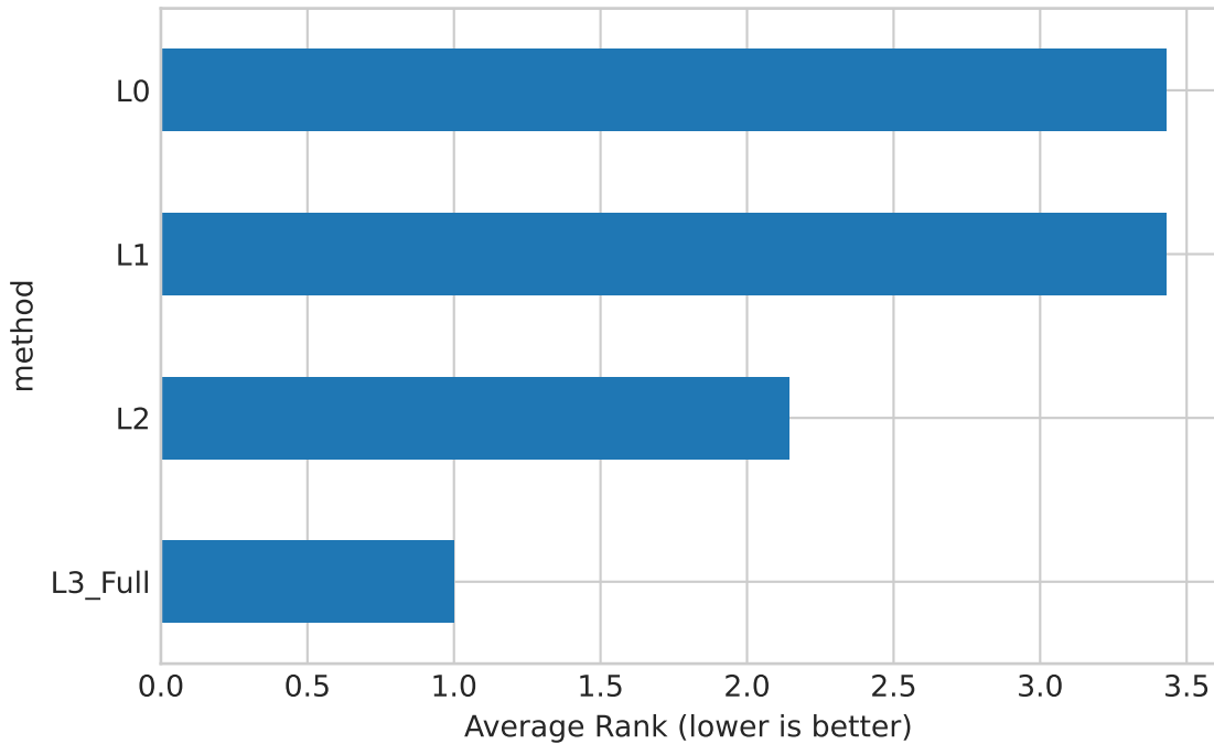
Average Rank Across Datasets
