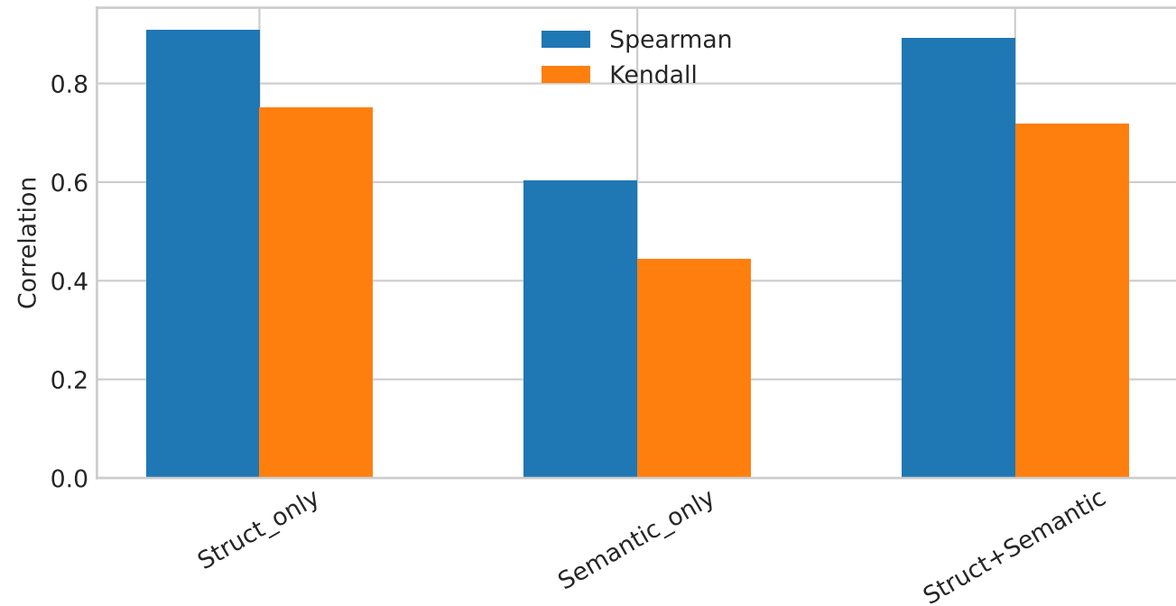
CiteSeer Ablation Study
